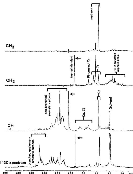
Figure 3. Quantitatively edited ^{13}\text{C} spectra using the DEPT pulse sequence.
