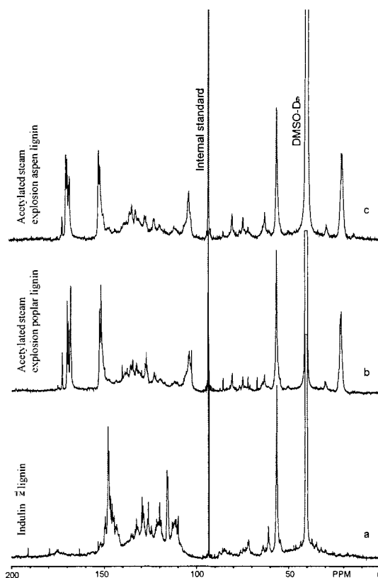
Figure 2. Quantitative ^{13}\text{C} NMR spectra of Round Robin lignins.
